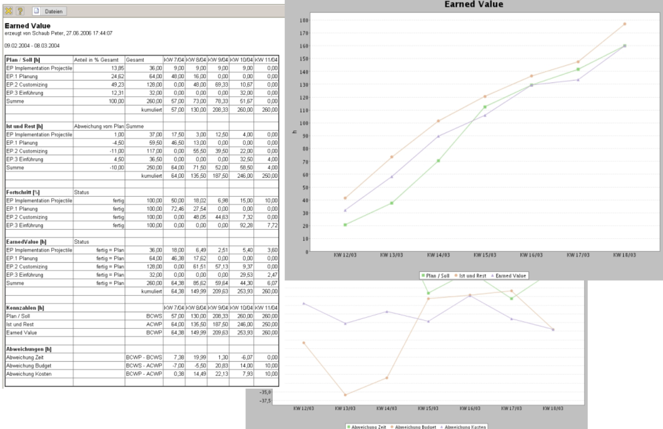
Abbildung 22: Earned-Value-Analyse
