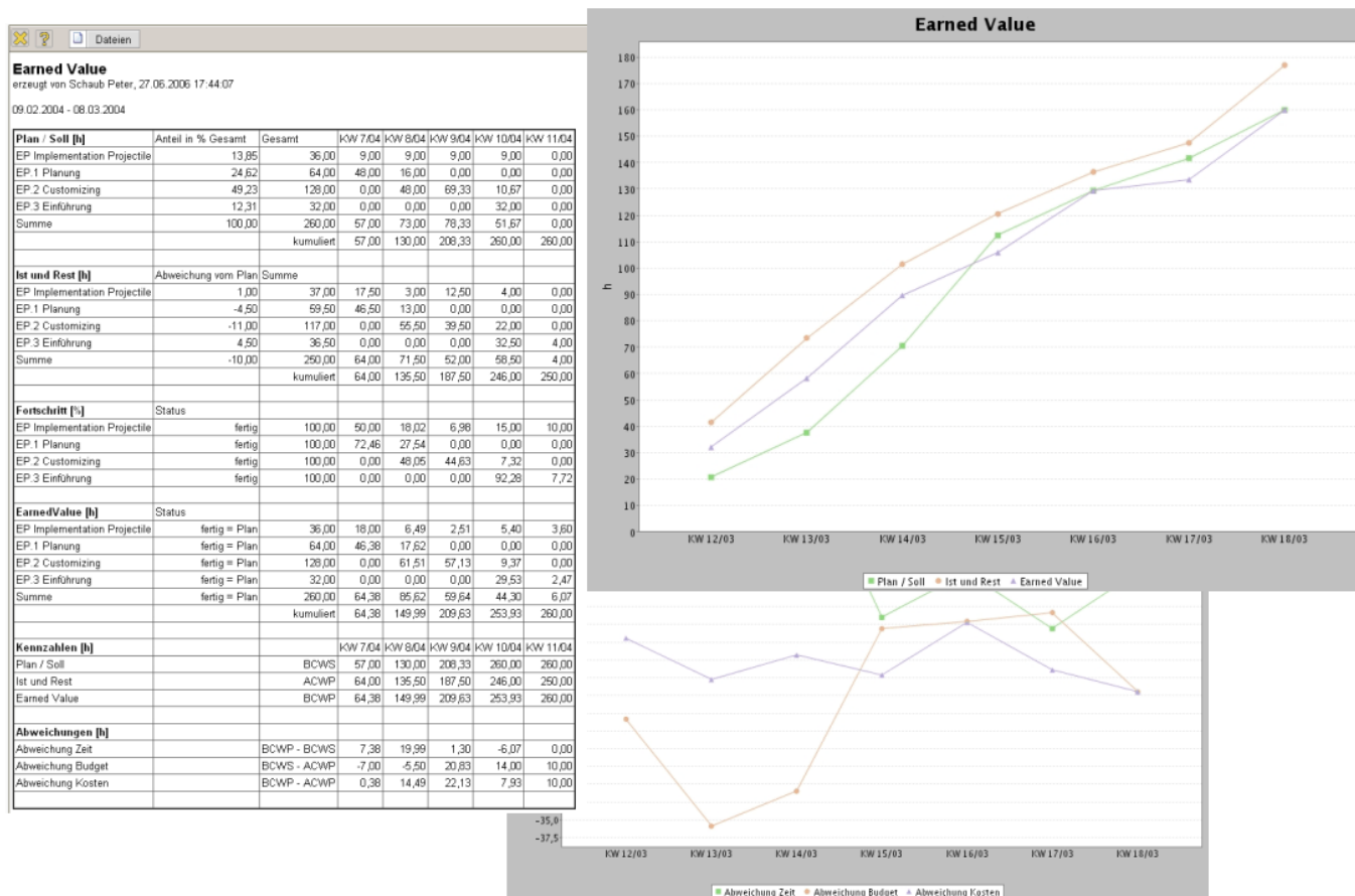
Abbildung 22: Earned-Value-Analyse
